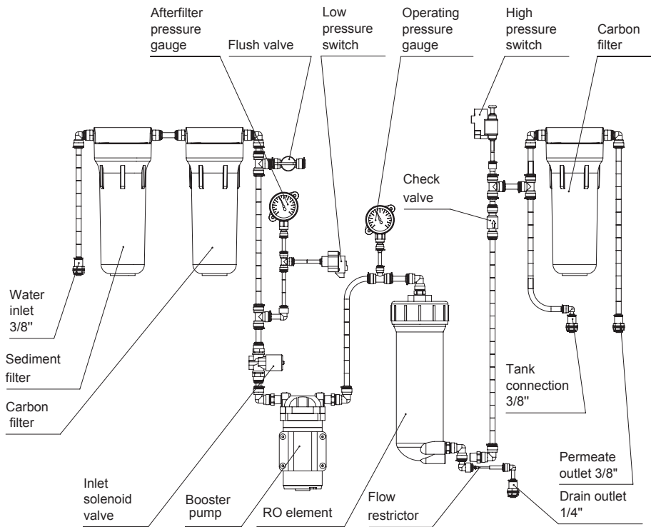
Figure 3. ROburst 1500 (Code: ROBUST1500ECO)
