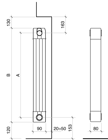
MEASURES EXPRESSED IN MILLIMETRES
