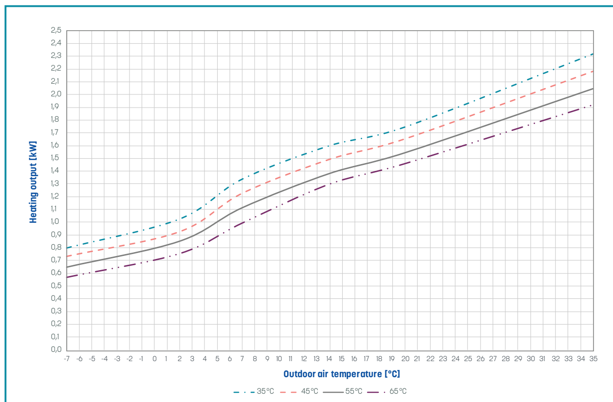
Chart: Heating output EN14511
