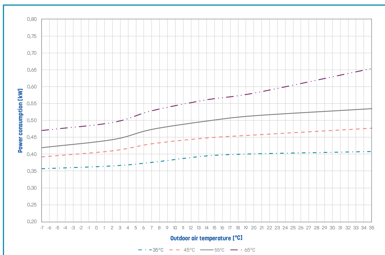
Chart: Power consumption EN14511
